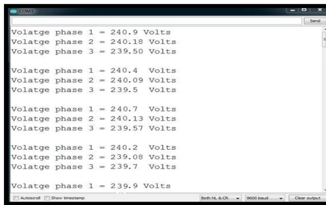
Figure. 17 Over Voltage obtain on Arduino
