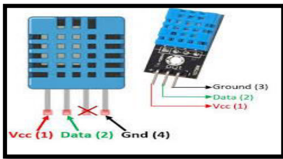
Figure. 4 Temperature Sensors (DHT 11)
