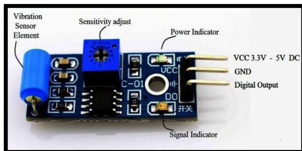
Figure 5 Vibration sensor (LM393)
