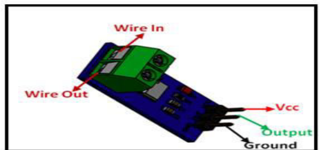
Figure 3 Current Sensors (ACS712)
