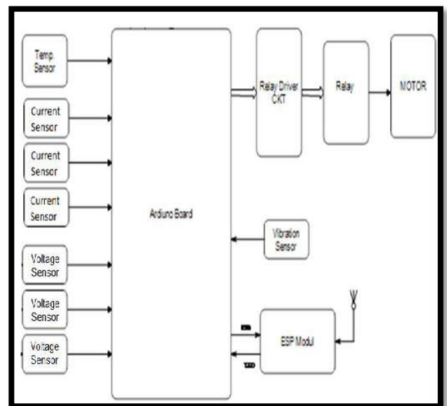
Fig 8 Block Diagram
