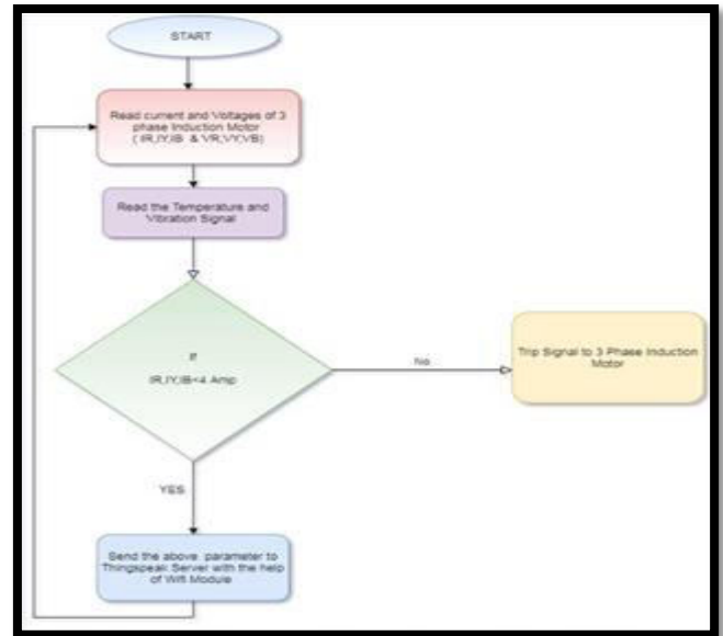
Figure 10 Flowcharts for Controlling from Motor Side. Steps for monitoring and controlling of 3 Phase Induction Motor from Motor Side
