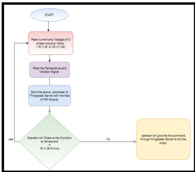
Figure.9 Flowcharts for Controlling from Remote Side Steps for monitoring and controlling of 3 Phase Induction Motor from Remote Side.
